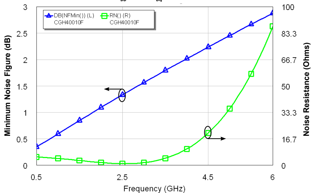
Simulated Minimum Noise Figure and Noise Resistance vs Frequency of the CGH40010F
